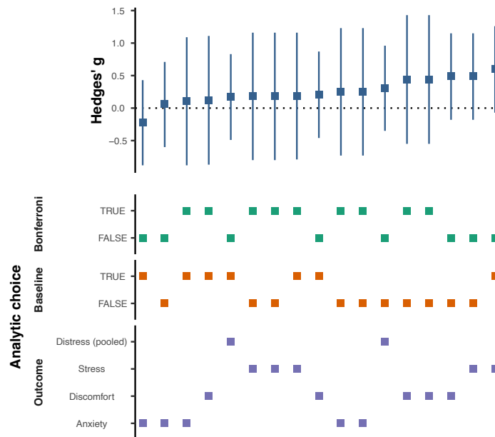
Figure 3. Multiverse plot for the replication study (Foody et al., 2015). Error bars represent 95% Confidence Intervals.
